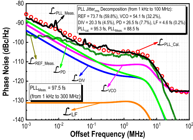
Fig. 20. Measured PLL phase noise, integrated jitter ( \sigma_{rms} ), and noise decomposition at 38.592 GHz.
