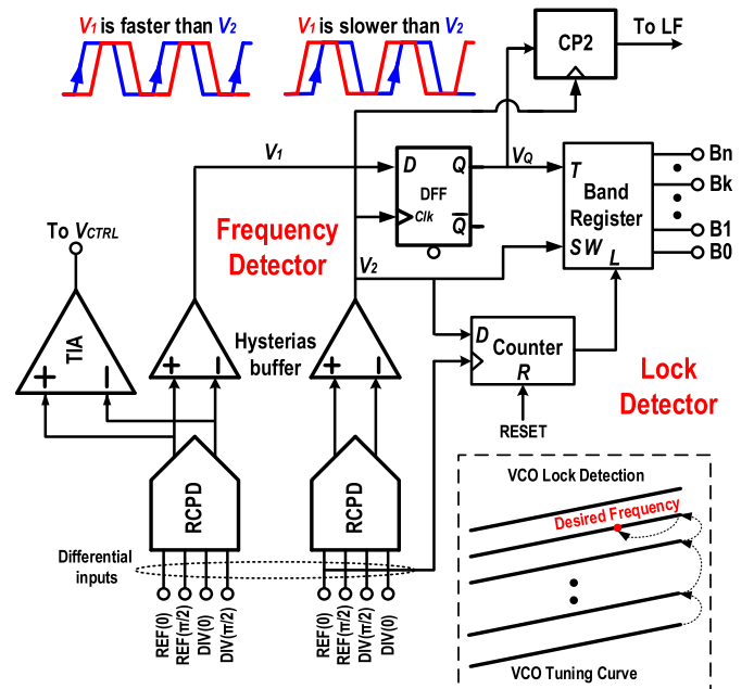
Fig. 9. RC-PFD evolved from RCPD.
