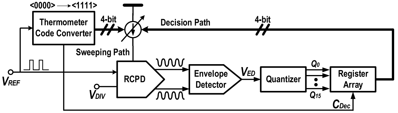
Fig. 7. Calibrator for ripple compensation.
