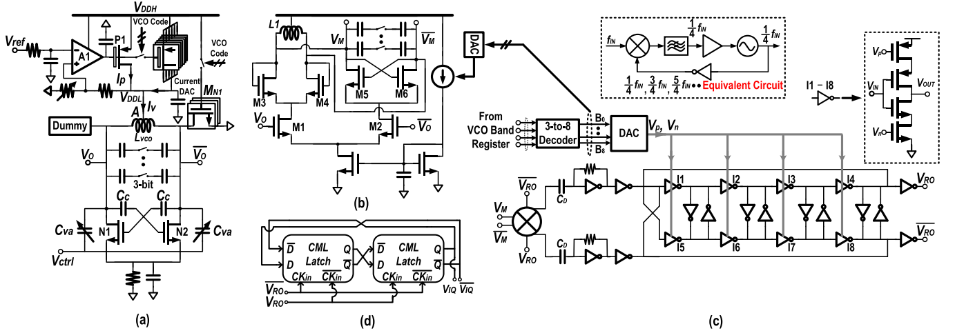
Fig. 10. MmW PLL building blocks includes (a) VCO (bias circuit not shown), (b) configurable Miller divider, (c) configurable ring-based ILFD, and (d) static divider generating I/Q signal for the RCPD performing ripple compensation.
