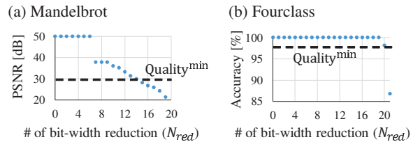
Fig. 6. The relation between N_{red} and Quality^{\min} .
