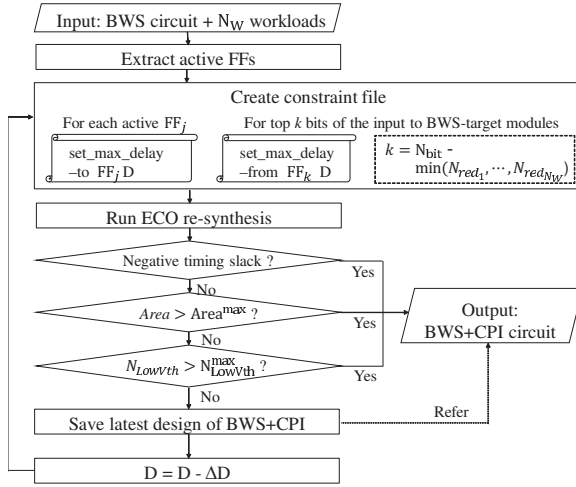
Fig. 4. Overview of the CPI flow.
