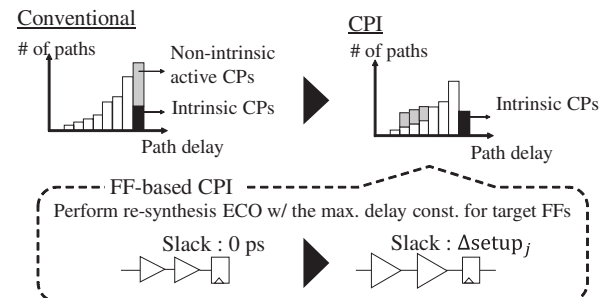
Fig. 3. Assumed FF-based CPI with re-synthesis.
