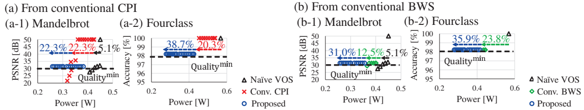
Fig. 7. Power saving effects of the proposed design from the conventional (a) CPI and (b) BWS. (a) From conventional CPI, the proposed design reduces the power dissipation thanks to BWS. (b) From conventional BWS, the proposed design mitigates the quality degradation slope thanks to CPI.
