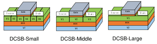
Fig. 5. Different configurations of sensitive volume size.
