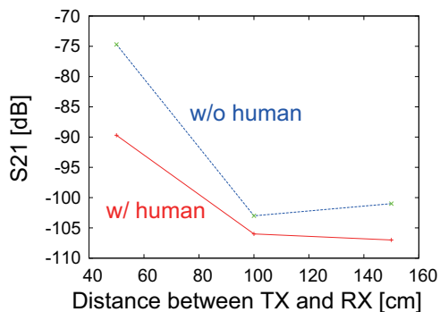
Fig. 7. Experimental result of horizontal attenuation.
