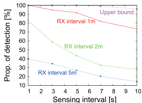
Fig. 9. Proportion of invader detection in case of Table I.
