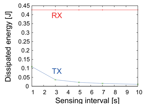
Fig. 10. Dissipated energy in case of Table I.
