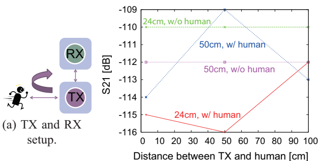
(b) Measured S21.
