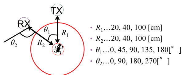
Fig. 8. Setup for collecting ultrasonic communication data.
