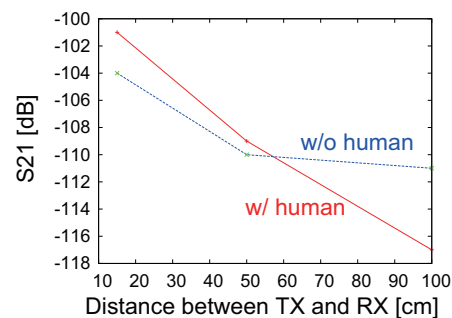
(b) Measured S21.
