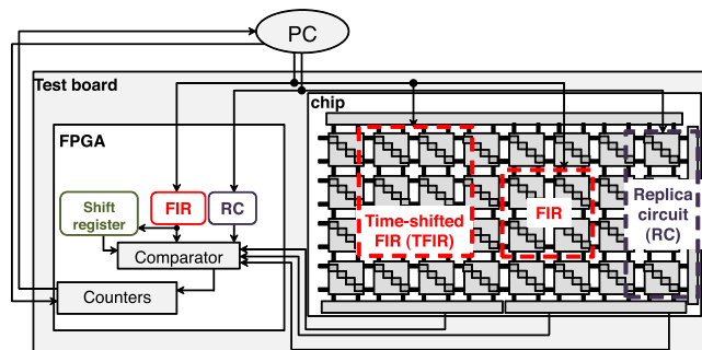
Fig. 4. Setup of the experiment.
