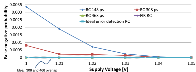
Fig. 8. False negative probability obtained from static variation experiments of RC. Note that the ideal, the RC 308 ps, and the RC 468 ps overlap.
