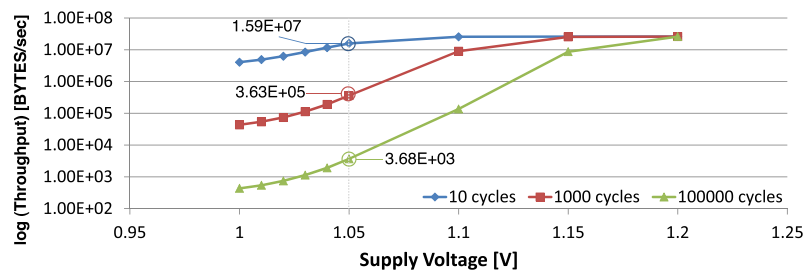
Fig. 9. Example demonstrating the effect of false negative probability on throughput.
