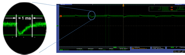
Fig. 11. Noise signal induced from a pulse of 3 V in amplitude.
