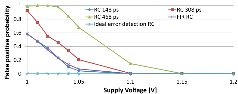
Fig. 7. False positive probability obtained from static variation experiment of RC.
