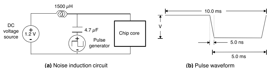
Fig. 6. Noise injection circuit and pulse waveform.
