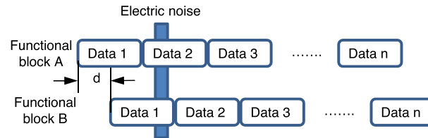
Fig. 1. Time diversity of redundant computation.
