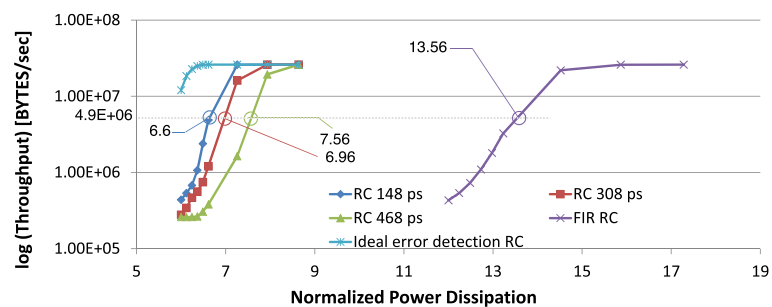
Fig. 10. Example demonstrating throughput vs. normalized dissipated power for each circuit.
