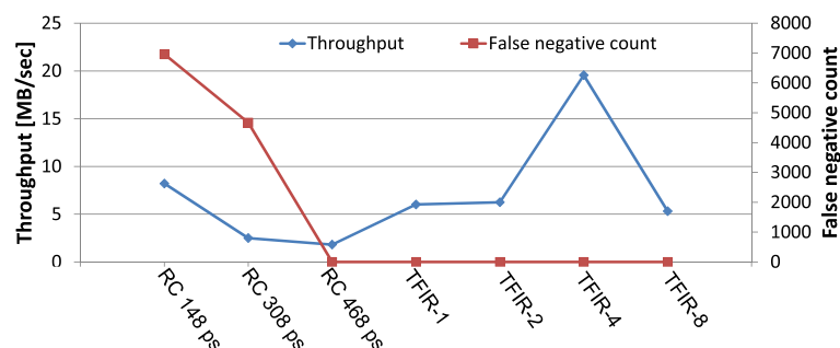
Fig. 12. Throughput and false negative count collected in the dynamic noise experiments.
