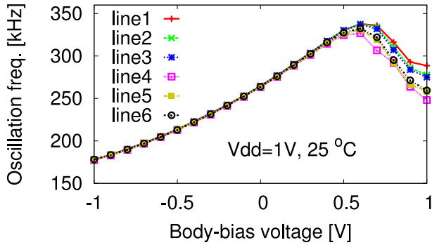
Figure 4: Measured frequency of ring oscillator at V_{dd}=1V and 25^{\circ}C .
