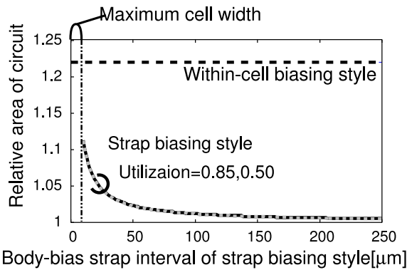
Figure 9: Area efficiency of strap biasing style with varied strap intervals (curved lines). Horizontal dashed line corresponds to within-cell biasing style.
