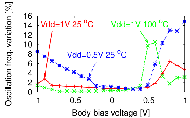
Figure 5: Frequency variation among lines at \{V_{dd}=1V, 25^{\circ}C\} , \{V_{dd}=1V, 100^{\circ}C\} and \{V_{dd}=0.5V, 25^{\circ}C\} .
