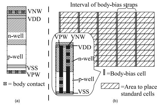
Figure 1: (a) Cell layout of within-cell biasing style. (b) Strap biasing style.
