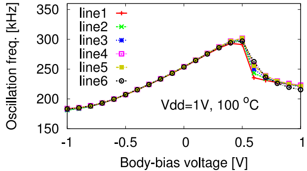
Figure 6: Measured frequency of ring oscillator at V_{dd}=1V and 100^{\circ}C .
