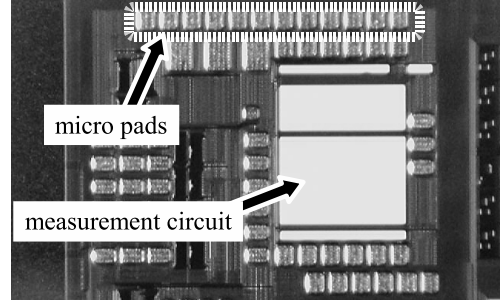
Figure 3: Micrograph of fabricated test chip.
