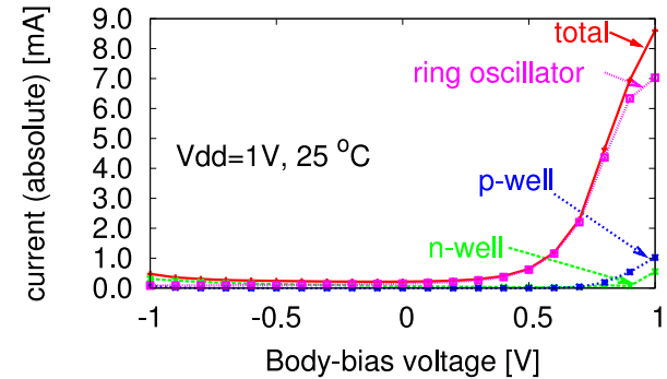
Figure 7: Measured current at V_{dd}=1V and 25^{\circ}C .
