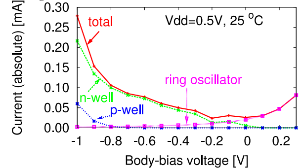
Figure 8: Measured current at V_{dd}=0.5V and 25^{\circ}C .
