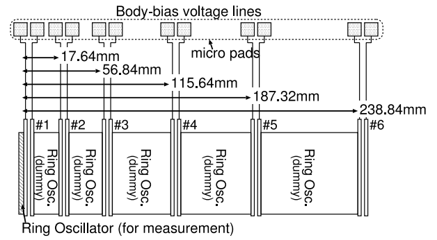
Figure 2: Structure of test circuit.
